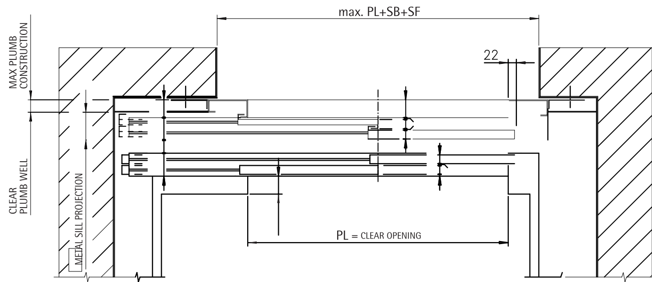
NICHE INSTALLATION
